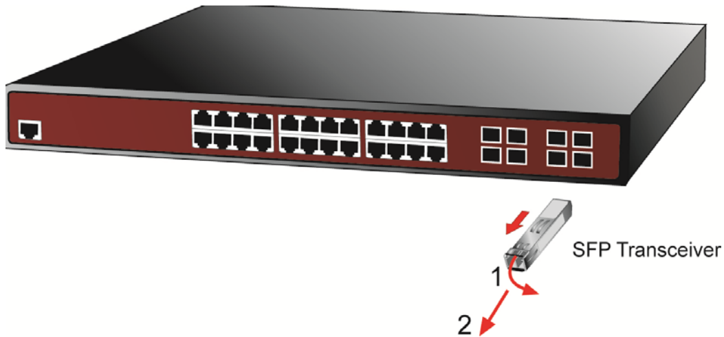
Figure 2-2-5: How to Pull Out the SFP/SFP+ Transceiver
