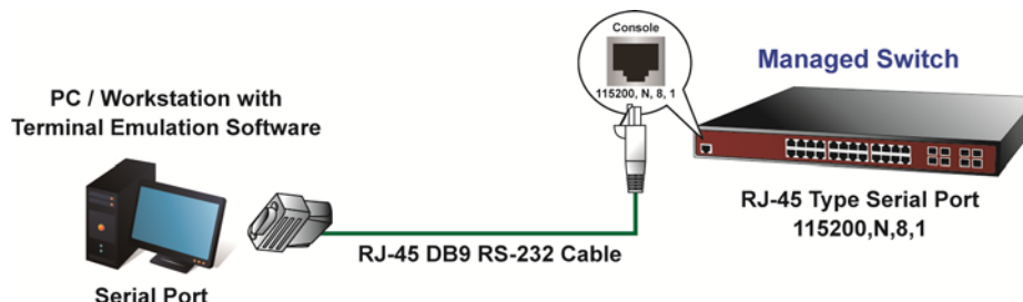
Figure 3-1-1: Console Management
