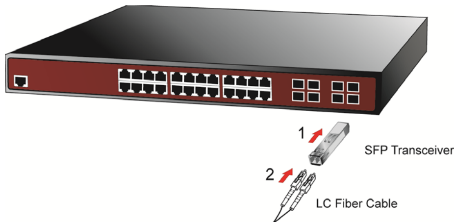
Figure 2-2-4: Plug-in the SFP/SFP+ Transceiver
