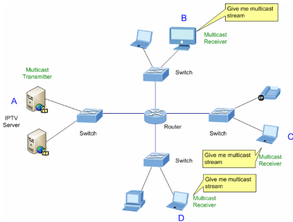
Figure 4-8-1: Multicast Service
