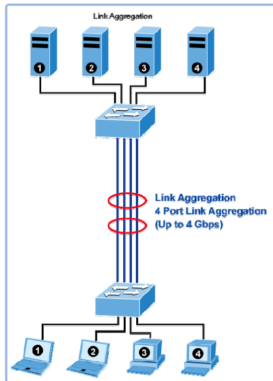
Figure 4-5-1: Link Aggregation
