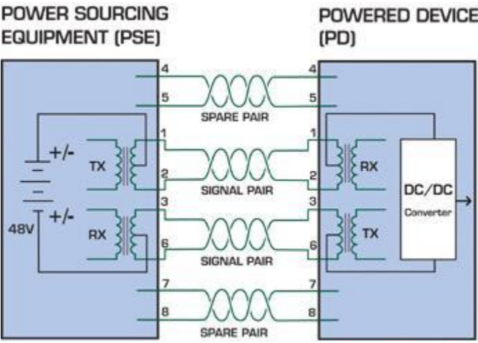
Figure 8-2: Power Supplied over the Data Pins
