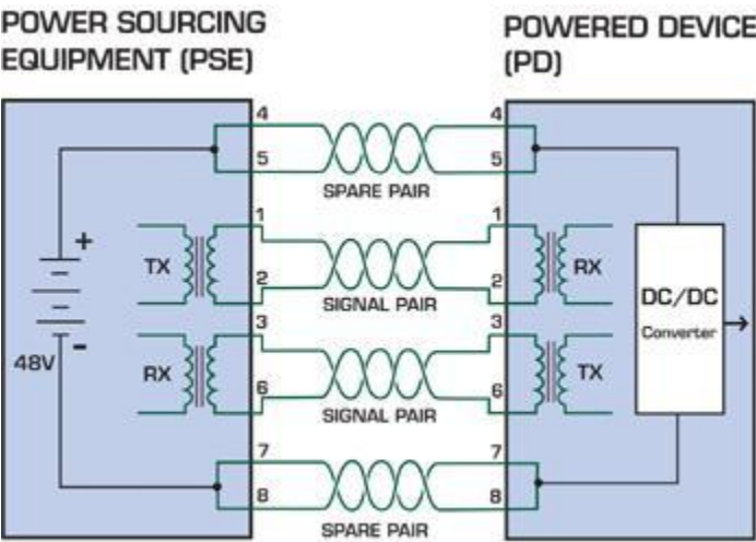
Figure 8-1: Power Supplied over the Spare Pins
